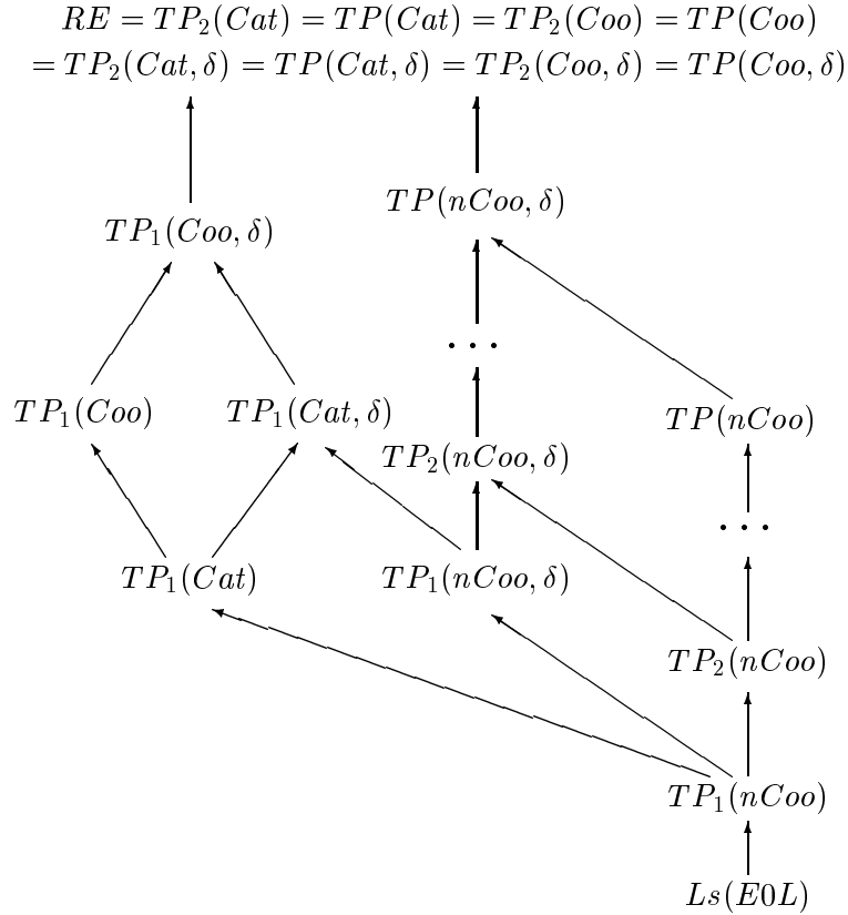
Figure 4. The hierarchy of the TP_n(\alpha) families.
